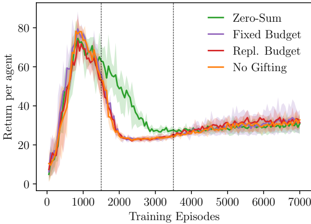
Figure 8: Return per agent when gifting and firing are disabled.
