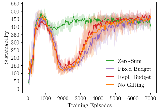
Figure 3: Sustainability for the three gifting mechanics and baseline, plotted throughout training. The zero-sum models see a small dip in performance before quickly recovering and converging to the final performance. The baseline and budgeted models only do so after suffering a great tragedy.
