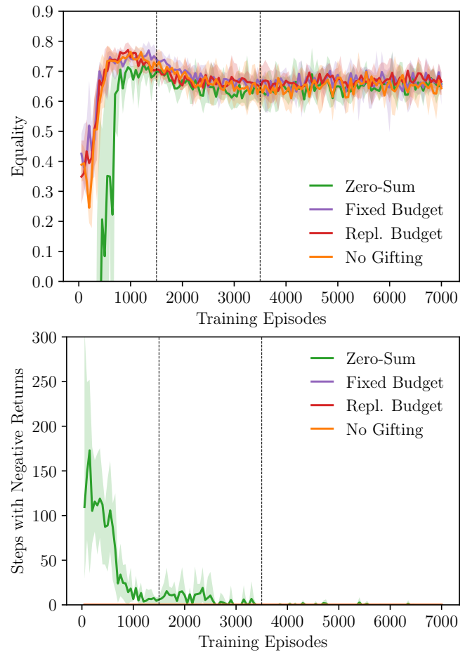
Figure 5: Top: Equality for the three gifting mechanics and baseline, plotted throughout training. Bottom: Average number of steps spend by zero-sum agents with a negative cumulative return up to that step. The low equality of the zero-sum model in early stages is due to agents gifting more than they gather and observing the resulting negative return. This is just a transient effect, and quickly all models converge to the same equality score.
